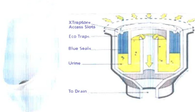
Waterless Urinal
